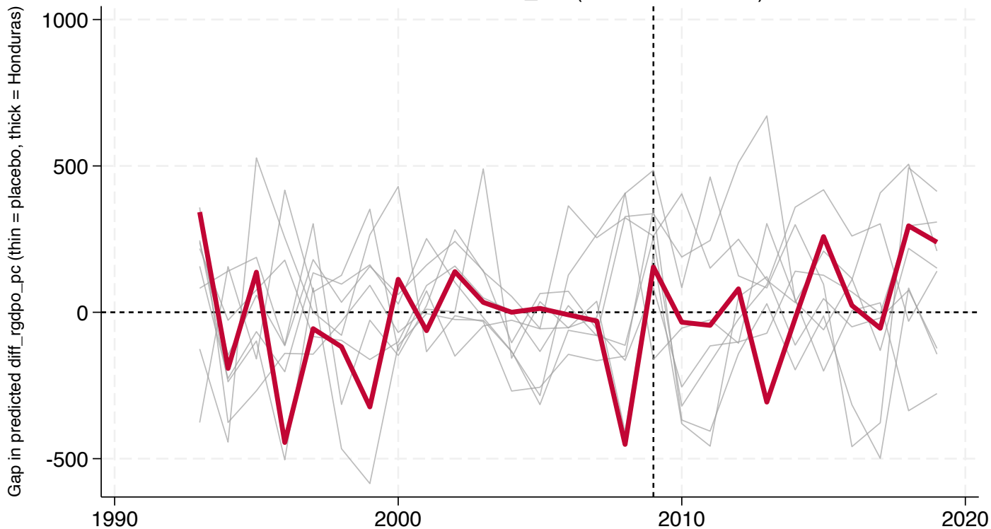
Latin America: naive_diff (outliers excluded)
